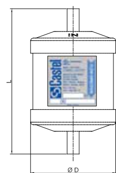
Solder connections
